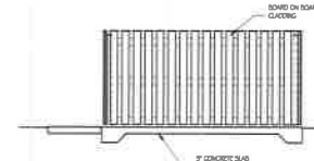
TRASH ENCLOSURE SIDE ELEVATION SCALE: 1/4" = 1'-0"
