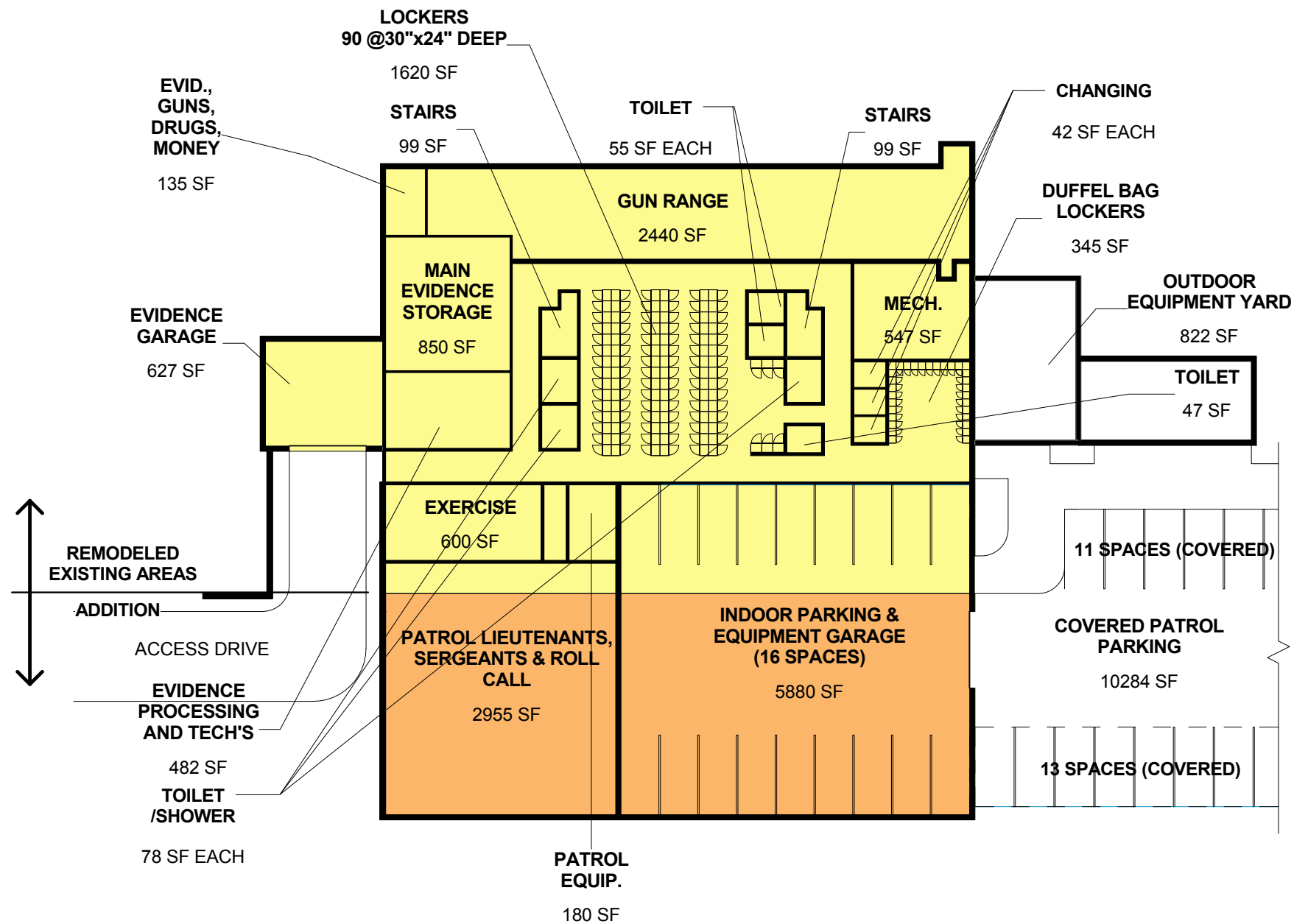
LOWER LEVEL FLOOR PLAN - CONCEPT 4
