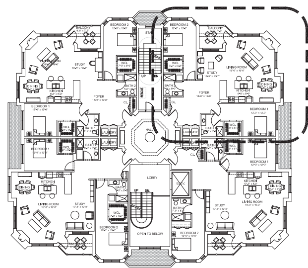
2 TYPICAL SECOND/THIRD FLOOR PLANS SCALE: 1/16"=1'-0"
