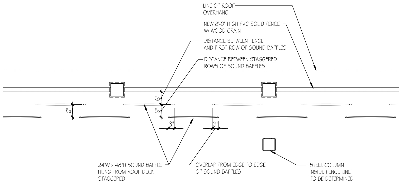
2 PLAN VIEW OF PERIMETER FENCE OF OUTDOOR AREA SCALE: 1/2" = 1'-0"
