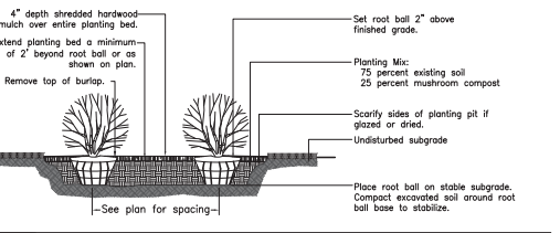
Detail Shrub Planting
