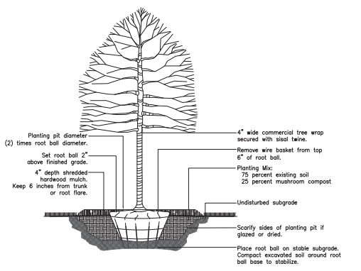
Detail Deciduous Tree Planting
