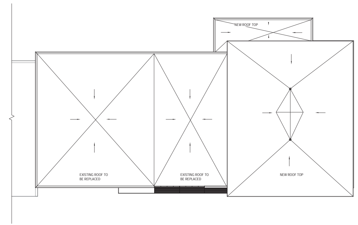
2 ROOF PLAN 1/16" = 1'-0"
