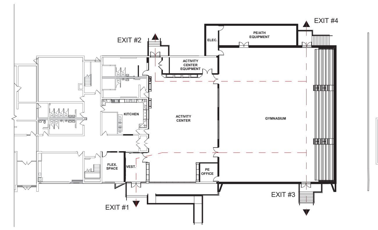
3 FIRST FLOOR EXIT PLAN 1/16" = 1'-0"
