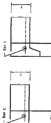
FLAT SLAB TOP JOINT CONFIGURATIONS FOR D = 36 (900) AND D = 4'-0" (1.22 m)
