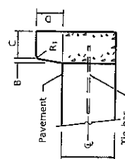
BARRIER CURB
