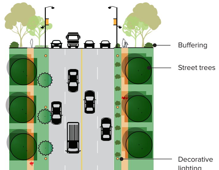
Proposed Streetscape
