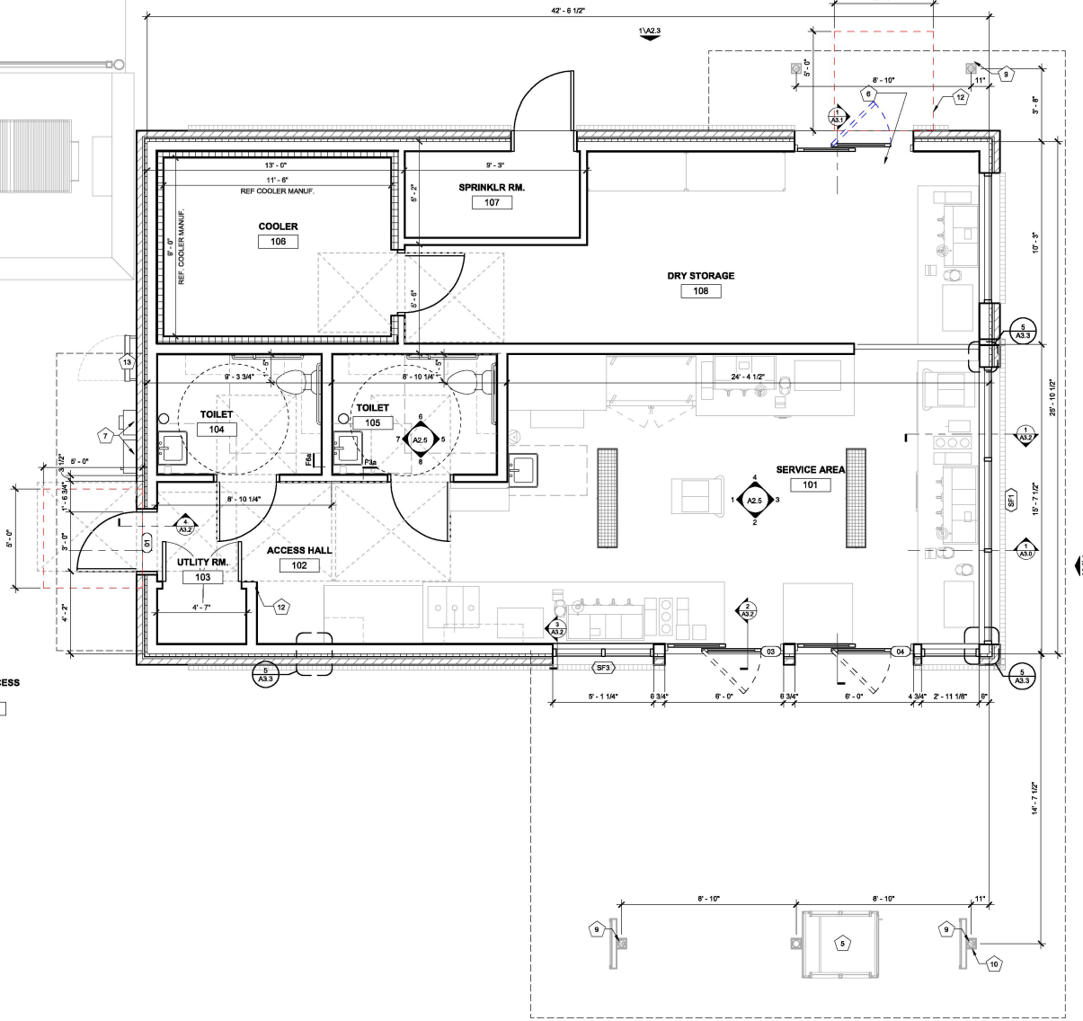
1 FLOOR PLAN 3/8" = 1'-0"
