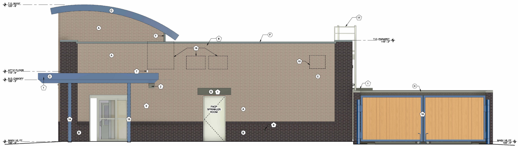
1 EXTERIOR ELEVATION - LEFT 3/8" = 1'-0"
