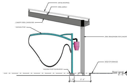
4 Canopy Section - Site Plan Approval A.101A 3/8" = 1'-0"
