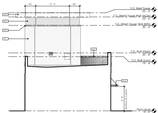
3 West Exterior Elevation (@ East Tower) - Site Plan Approval A.101A 3/16" = 1'-0"
